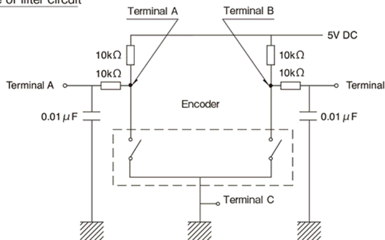
Example of filter circuit
